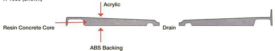
Cross section for Ballast™ shower base K-1935 (Shown)
